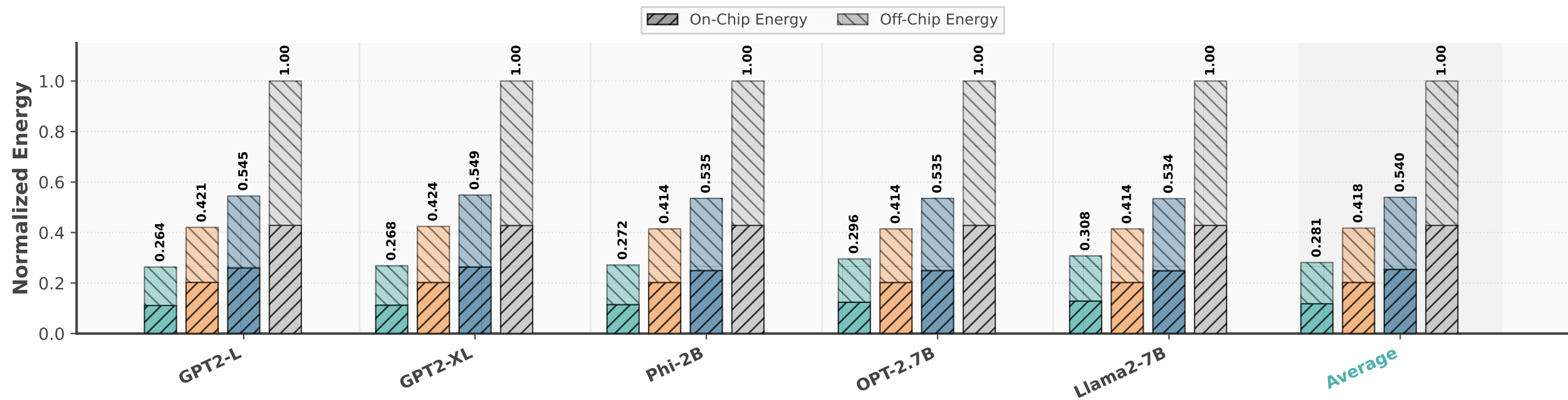
(b) Energy Consumption Comparison
