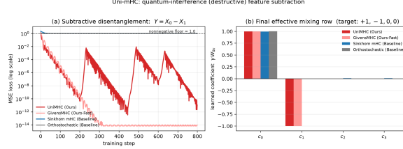
Figure 2: Subtractive disentanglement ( Y = X_0 - X_1 ). (a) Uni-mHC and GivensMHC reach machine precision; non-negative baselines plateau at the impossibility floor (Prop. 2). (b) Learned coefficients \gamma W_{0k} : phase interference yields the exact (+1, -1, 0, 0) pattern; non-negative mixers degenerate to a pure copy (+1, 0, 0, 0) .
