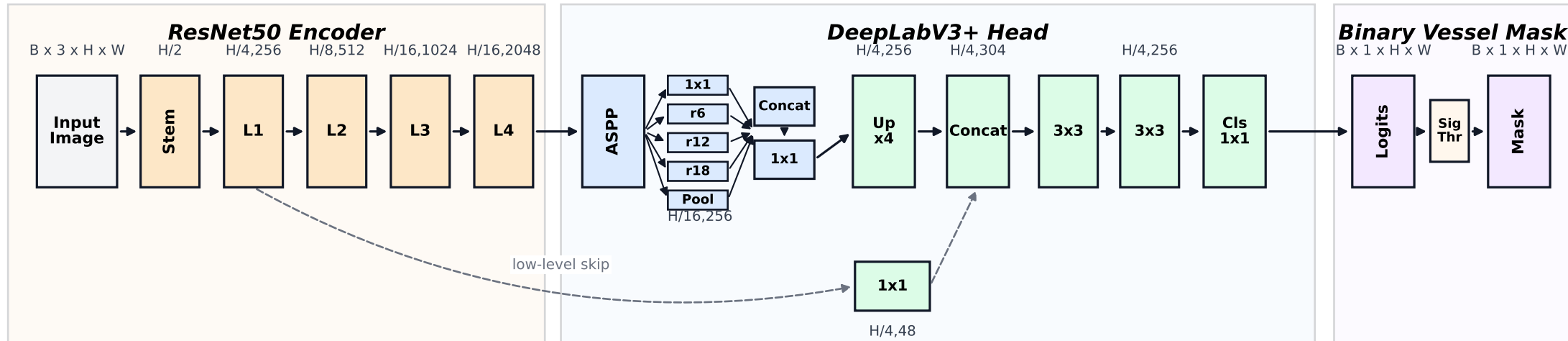
Figure X. Compact architecture of DeepLabV3+-ResNet50. ResNet50 extracts features; DeepLabV3+ uses ASPP and a low-level skip decoder to produce a binary vessel mask.
