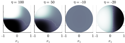
\rho(x; 100)
