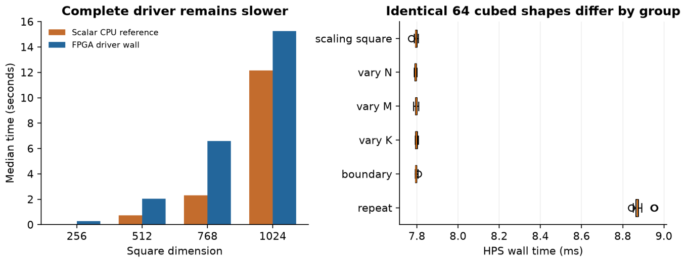
Figure 5 Left: independent median CPU reference and FPGA driver times in the large suite. Right: distributions of 30 measured runs for identical 64 cubed shapes in original suite order; boxes show quartiles and the line shows the median.
