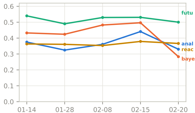
Brier vs truth (lower is better) — parallel
