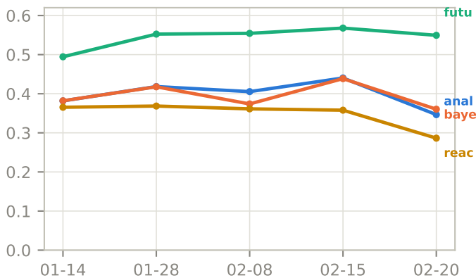
Brier vs truth (lower is better) — sequential
