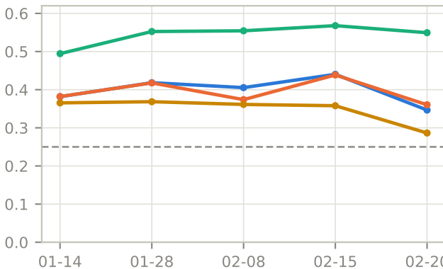
Brier vs truth (lower is better) — sequential
