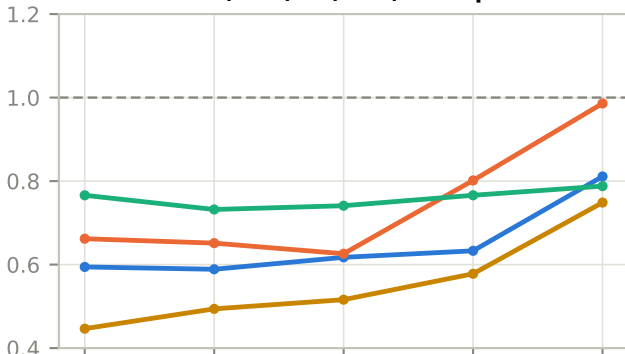
Coherence P(\text{USA})+P(\text{CAN}) — sequential
