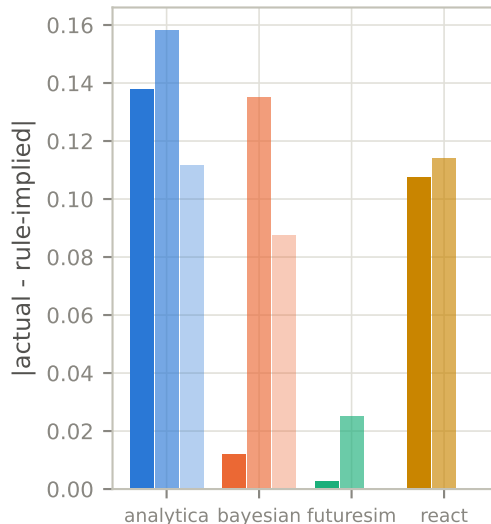
Rule-compliance gap (dark to light: toward, against, placebo)
