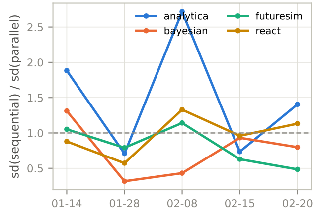
Is history a variance reducer?
