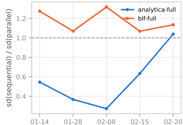
Is history a variance reducer? (real code)
