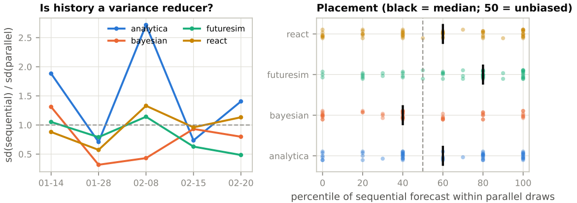
Figure 8: Left: stabilisation ratio \text{sd}(\text{SEQ})/\text{sd}(\text{PAR}) . History acts as a variance reducer where the ratio sits below 1; analytica 's ratio above 1 on several dates is path dependence—rollouts diverge because their own early draws differed. Right: placement of every sequential forecast within its date's fresh-eyes distribution; futuresim 's median sits at the 80th percentile (anchored high), bayesian 's at the 40th.
