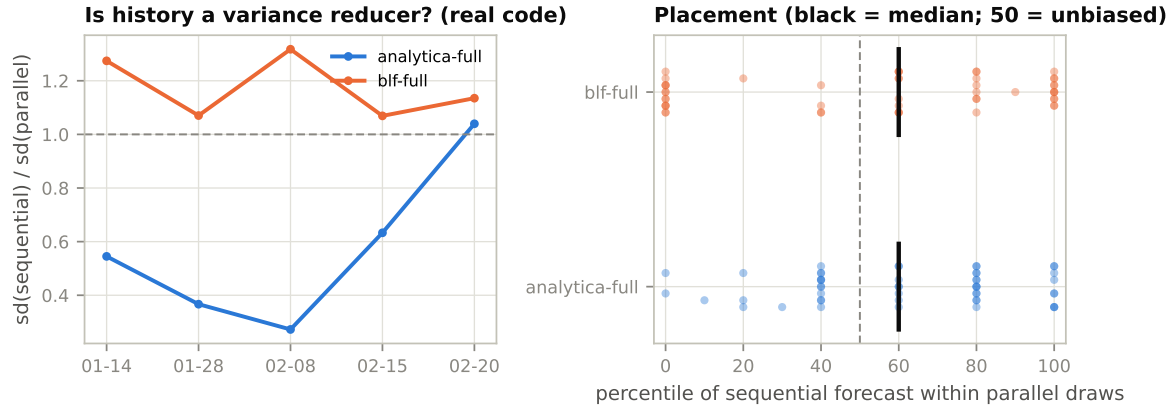
Figure 14: Stabilisation and placement, real tier. analytica-full sits far below 1 through mid-window: carrying the tree strongly reduces cross-rollout variance. blf-full sits above 1 throughout—carrying the belief state does not reduce variance at all.
