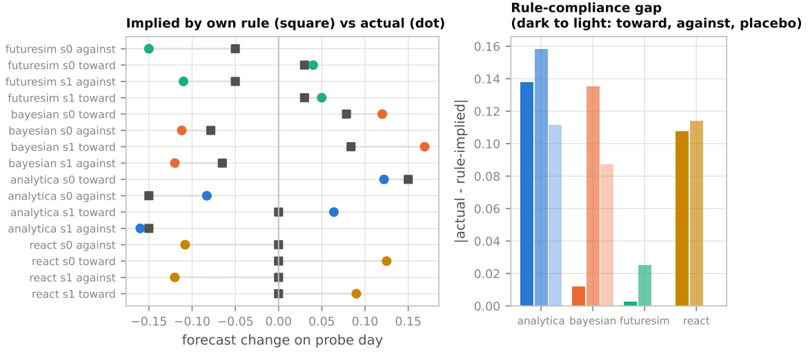
Figure 18: Left: single-coordinate implied change (square) vs actual change (dot) for every directional probe. Right: the multi-coordinate rule-compliance gap |p_{\text{actual}} - p_{\text{rule}}| by condition. futuresim 's gaps are \leq 0.04 : handed the evidence, it computes with its recovered structure almost exactly. react 's program implies zero response in every cell while the live harness moved \pm 0.09 – 0.13 : its updates use machinery its recoverable structure does not contain.
