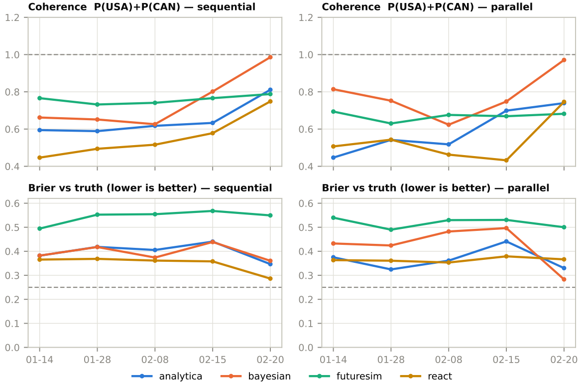
Figure 9: Coherence and accuracy by condition. Top: P_{USA}+P_{CAN} should approach 1 by the semifinal (dashed). Bottom: plain Brier against the resolved outcomes, pooled over the pair; the dashed line is 0.25, the constant- \frac{1}{2} forecaster.
