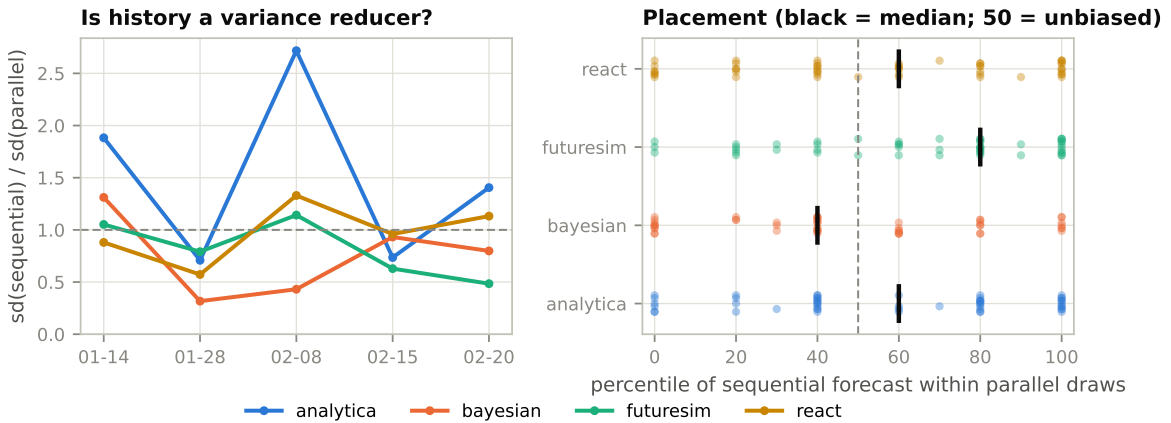
Figure 8: Left: stabilisation ratio \text{sd}(\text{SEQ})/\text{sd}(\text{PAR}) . History acts as a variance reducer where the ratio sits below 1; analytica 's ratio above 1 on several dates is path dependence—rollouts diverge because their own early draws differed. Right: placement of every sequential forecast within its date's fresh-eyes distribution; futuresim 's median sits at the 80th percentile (anchored high), bayesian 's at the 40th.
