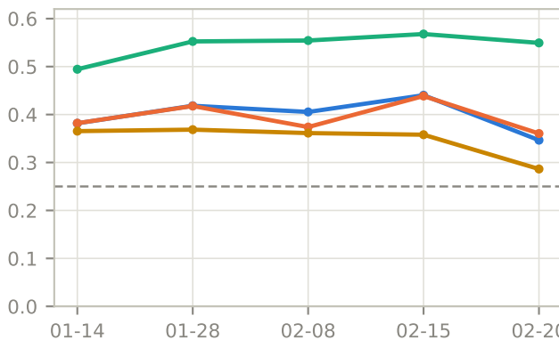
Brier vs truth (lower is better) — sequential
