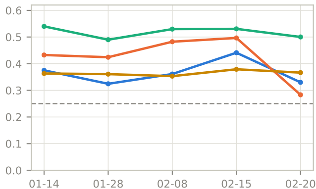
Brier vs truth (lower is better) — parallel
