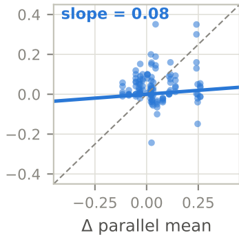
analytica-full
