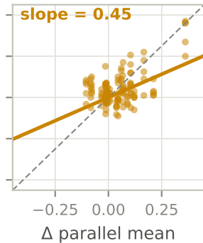
react
