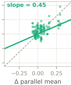
futuresim-full
