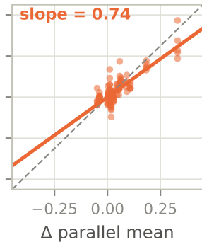
blf-full
