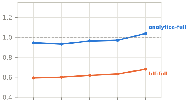
Brier vs truth (lower is better) — sequential
