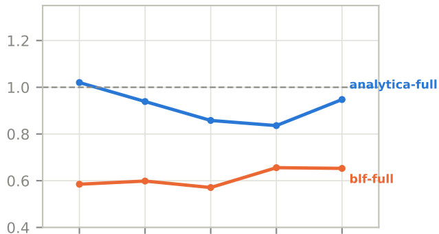
Brier vs truth (lower is better) — parallel
