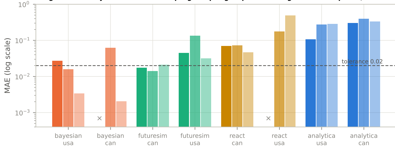
Program recovery — one literal-free program per group. Darker→lighter: in-sample fit, blind sample holdout, blind temporal holdout
