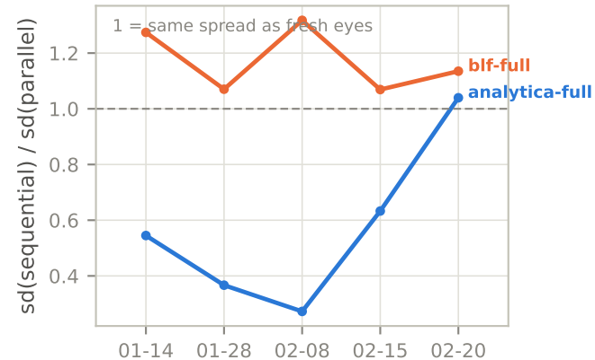
Is history a variance reducer? (real code)
