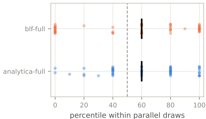
Coherence P(USA)+P(CAN) - parallel
