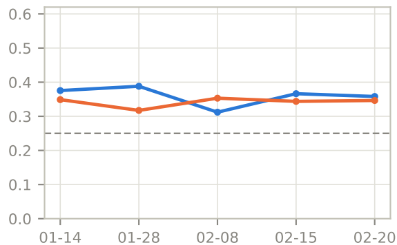
Brier vs truth (lower is better) - parallel
