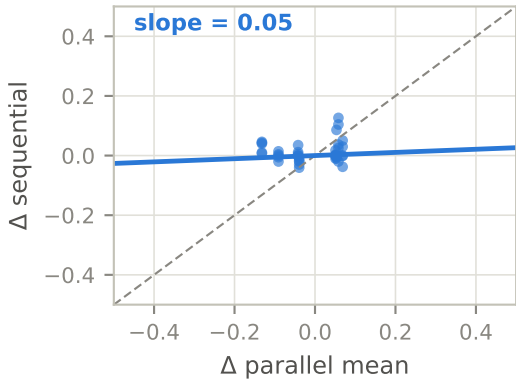
analytica-full
