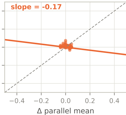
blf-full
