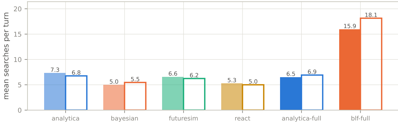
Search effort — filled: sequential, outlined: parallel (solid fill = real orchestration code)
