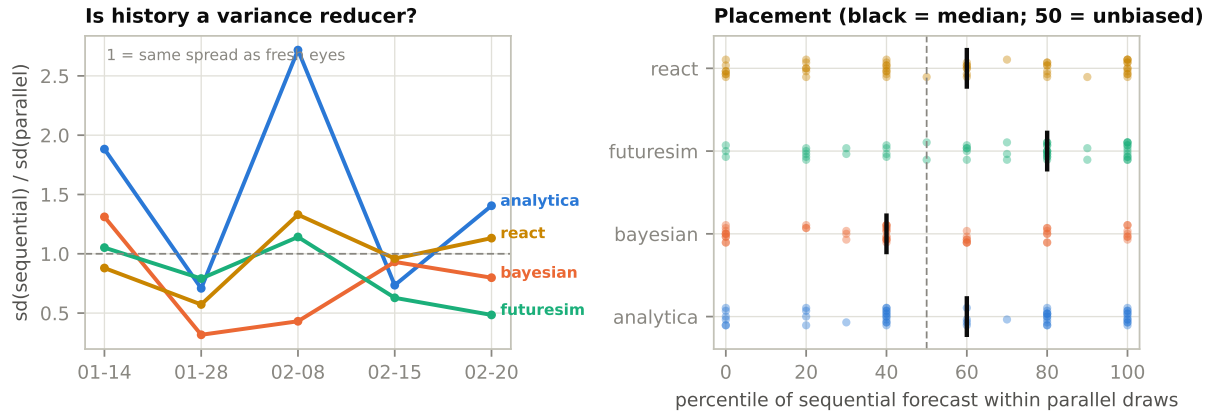
Figure 4: Left: stabilisation ratio \text{sd}(\text{SEQ})/\text{sd}(\text{PAR}) . History acts as a variance reducer where the ratio sits below 1 ( futuresim , react ); analytica ’s ratio above 1 on several dates is path dependence—rollouts diverge because their own early draws differed. Right: placement of every sequential forecast within its date’s fresh-eyes distribution; futuresim ’s median sits at the 80th percentile (anchored high), bayesian ’s at the 40th.
