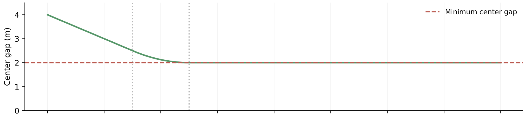
(c) B reaches 10 m at 8s; alone: 5s. No stopped waiting.
