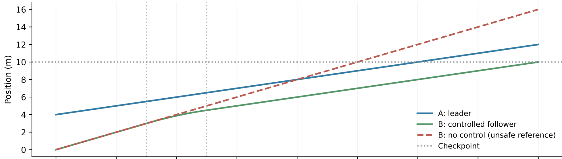
(a) A faster follower slows down before reaching the leader
