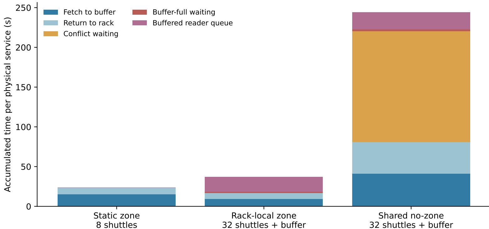
Where transport-side time goes
