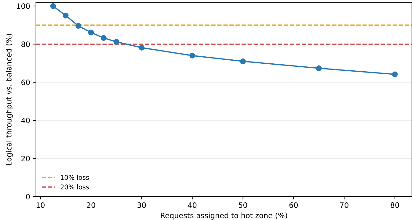
Static-zone throughput under merged request skew
