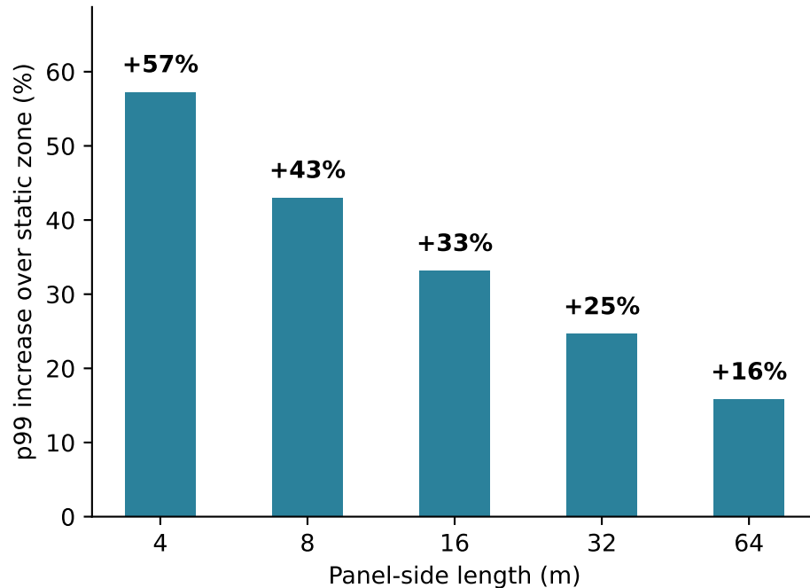
(b) No-zone tail-latency penalty
