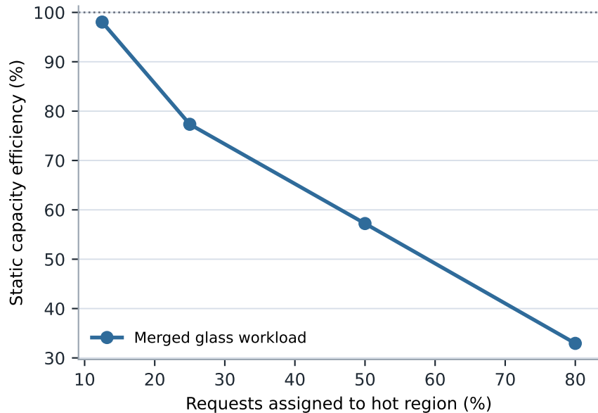
Cold-zone capacity becomes stranded
