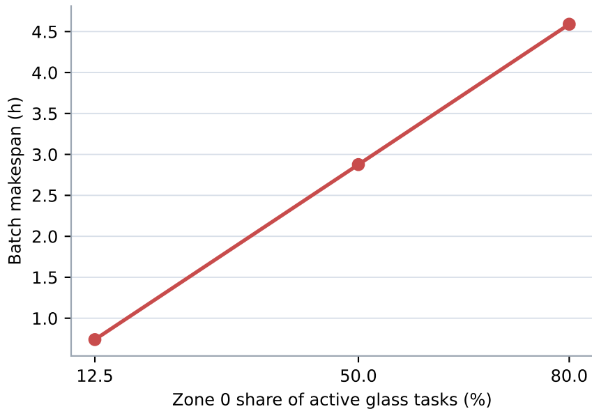
A hotspot stretches the fixed owner's queue
