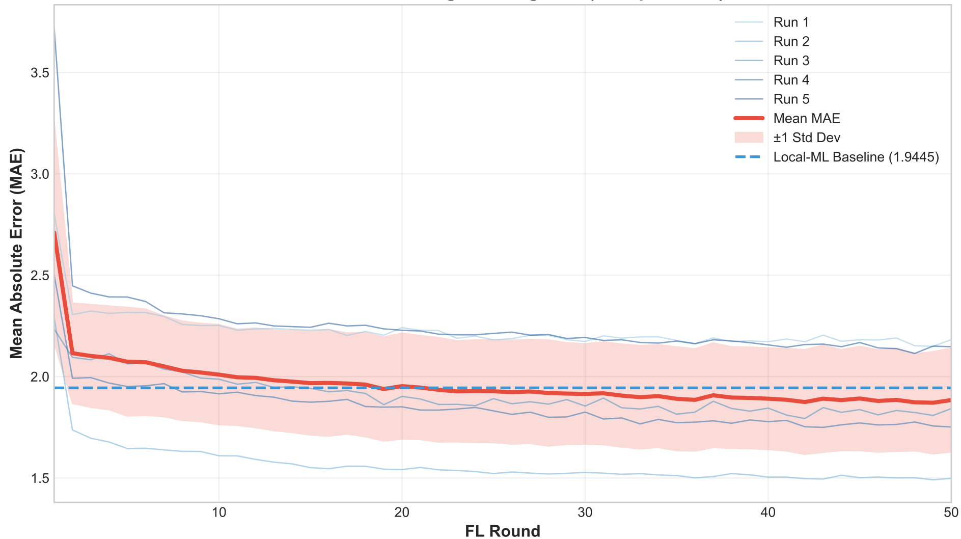
Federated Learning Convergence (Multiple Runs)
