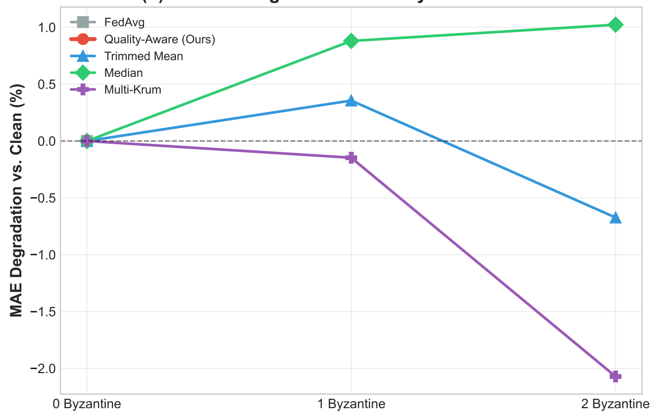
(b) Relative Degradation from Byzantine Attacks
