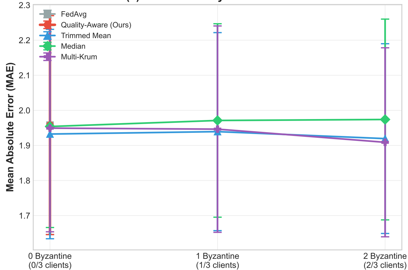
(a) MAE Under Byzantine Attacks
