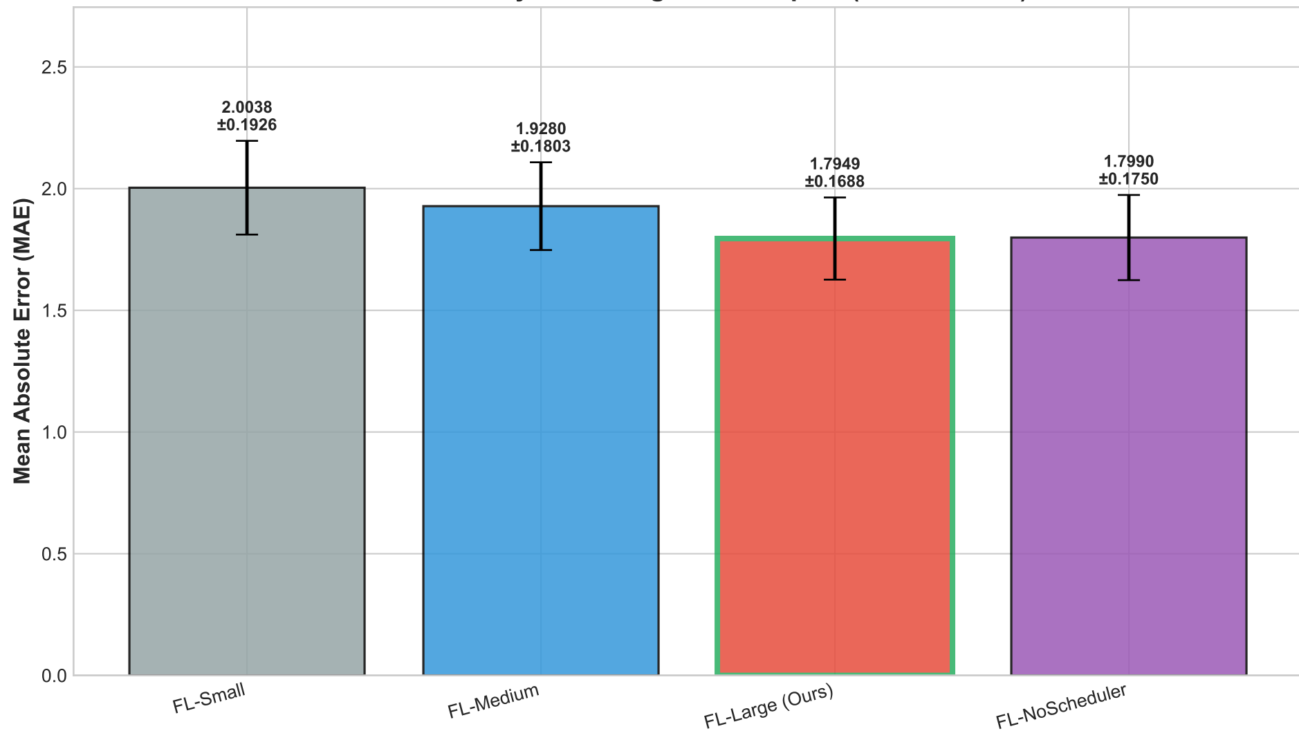
Ablation Study: FL Configuration Impact (5 seeds each)
