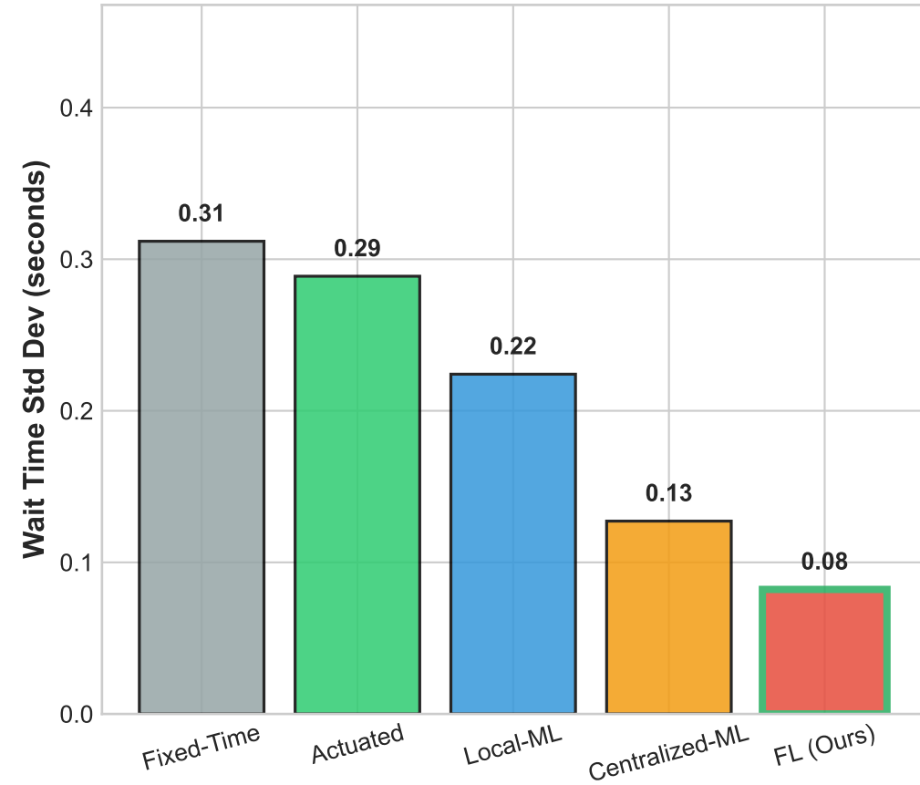
(c) Stability (Lower is Better)
