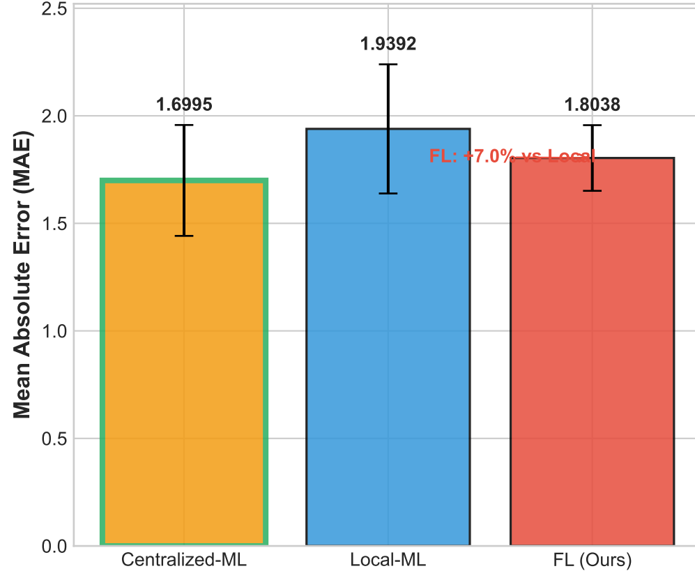
(b) Prediction Accuracy
