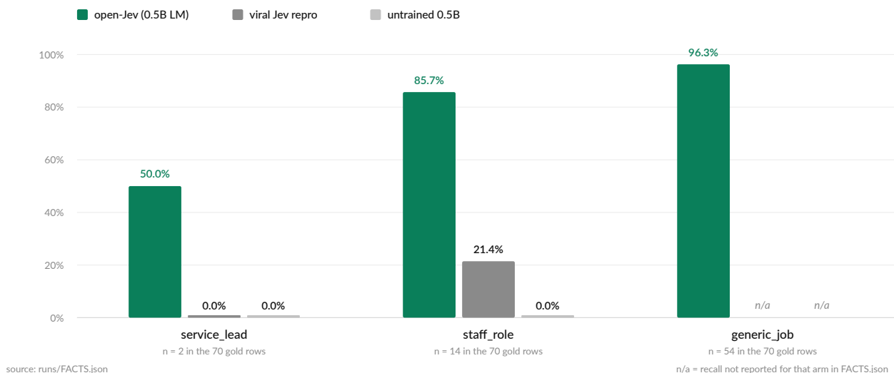
Figure 3. Per-class recall on the same 70 rows. The whole difficulty of this task lives in the two middle bars of the left pair.
