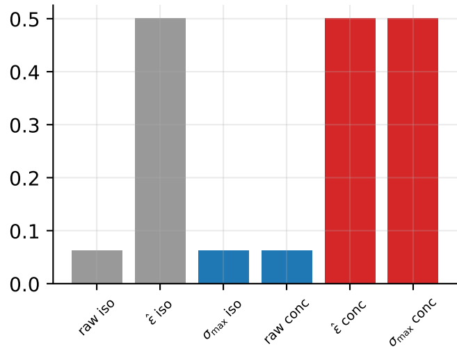
raw understates concentrated \sigma_{\max} by \sqrt{\hat{\epsilon}} \hat{\epsilon} is conservative for both
