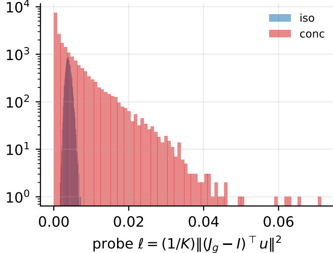
probe sees the SAME energy
