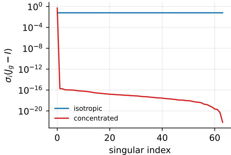
matched energy \|E\|_F = 0.5
