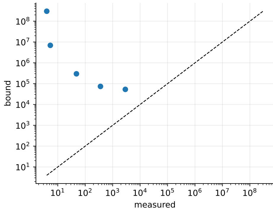
bound above measurement (valid, loose)
