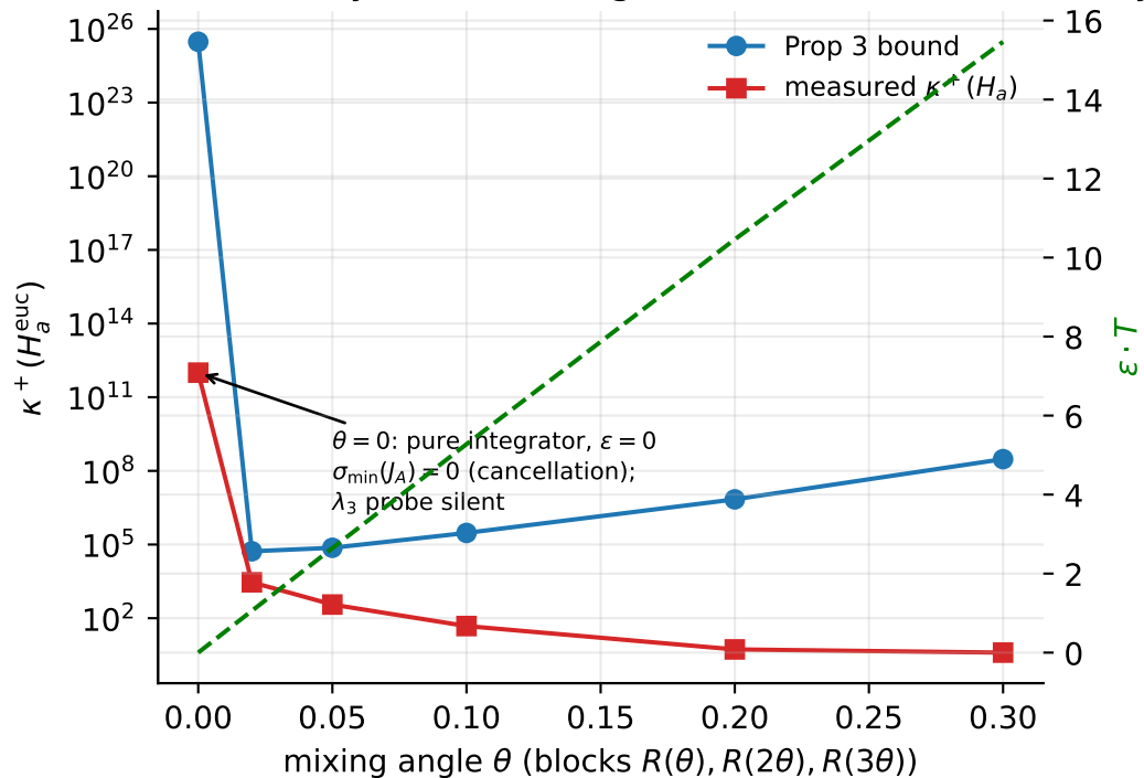
G1: controllability needs mixing; Theorem 2 needs isometry
