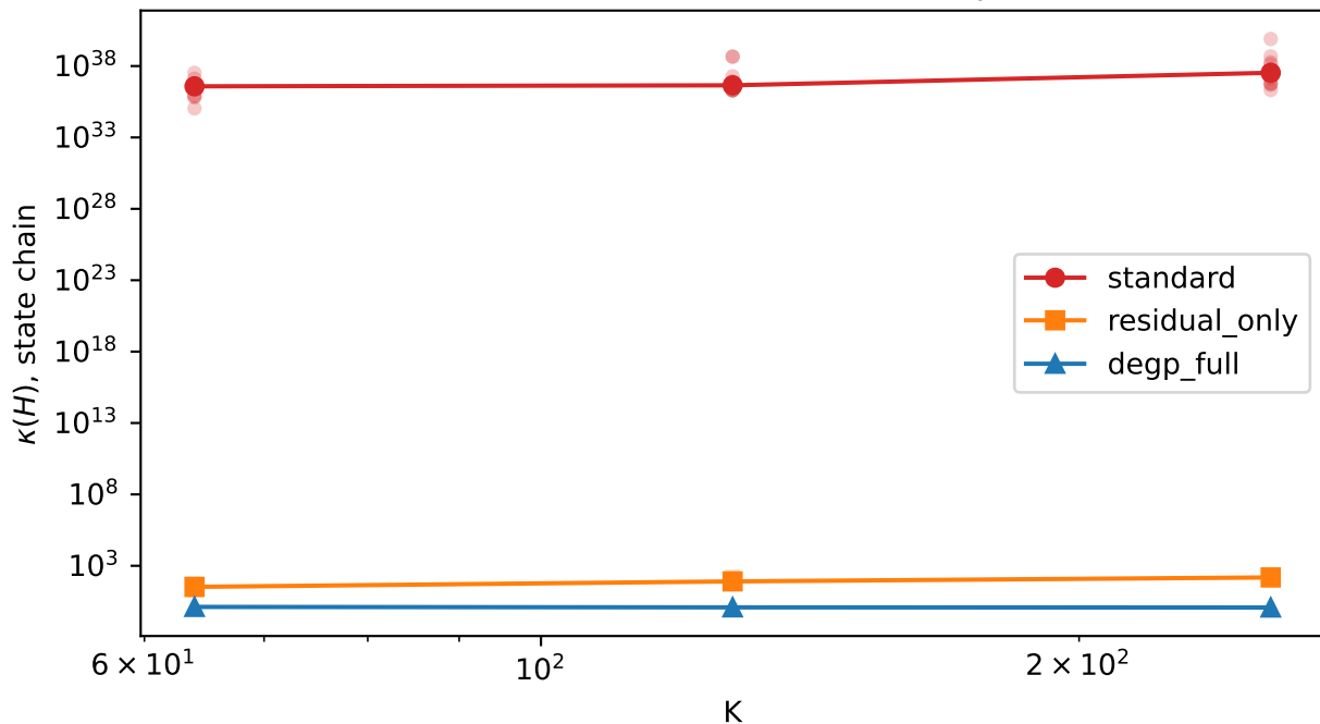
Experiment 2, K-sweep: DEGP flat, standard uncontrolled (R1 TOST verdicts in Cell B4 output)
