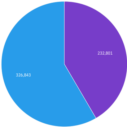
gender by usertype and gender
