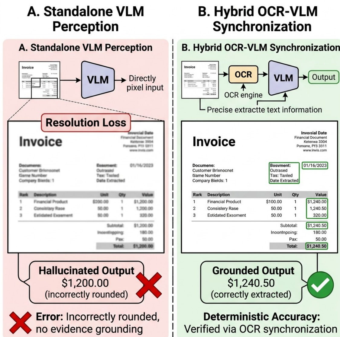
Figure 7.6: Visual Case Study and Model Response Screenshots demonstrating VLM Resolution-Loss vs. Hybrid Precision (Source: Adapted from [31])
