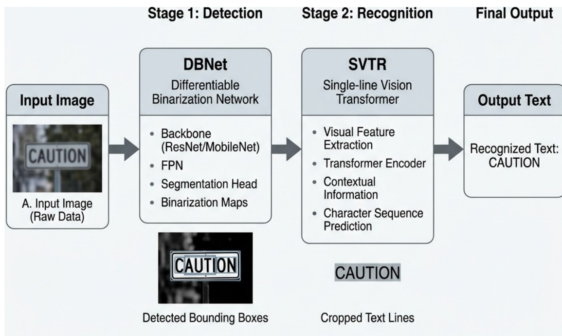
Figure 2.2: PaddleOCR Advanced Multi-Stage Architecture (DBNet + SVTR) (Source: Adapted from [4])
