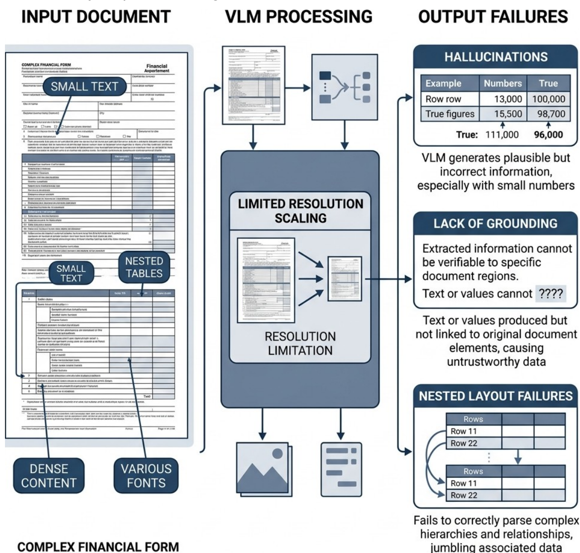
Figure 2.4: VLM Projection Layer and Resolution Constraints (Source: Adapted from [31])
