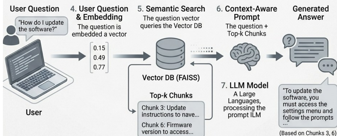
Figure 2.5: Semantic Embedding and Vector Storage Workflow (Source: Own elaboration)
