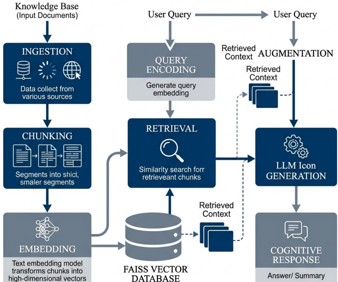
Figure 3.1: Minimal RAG Retrieval Principle (Source: Own elaboration)
