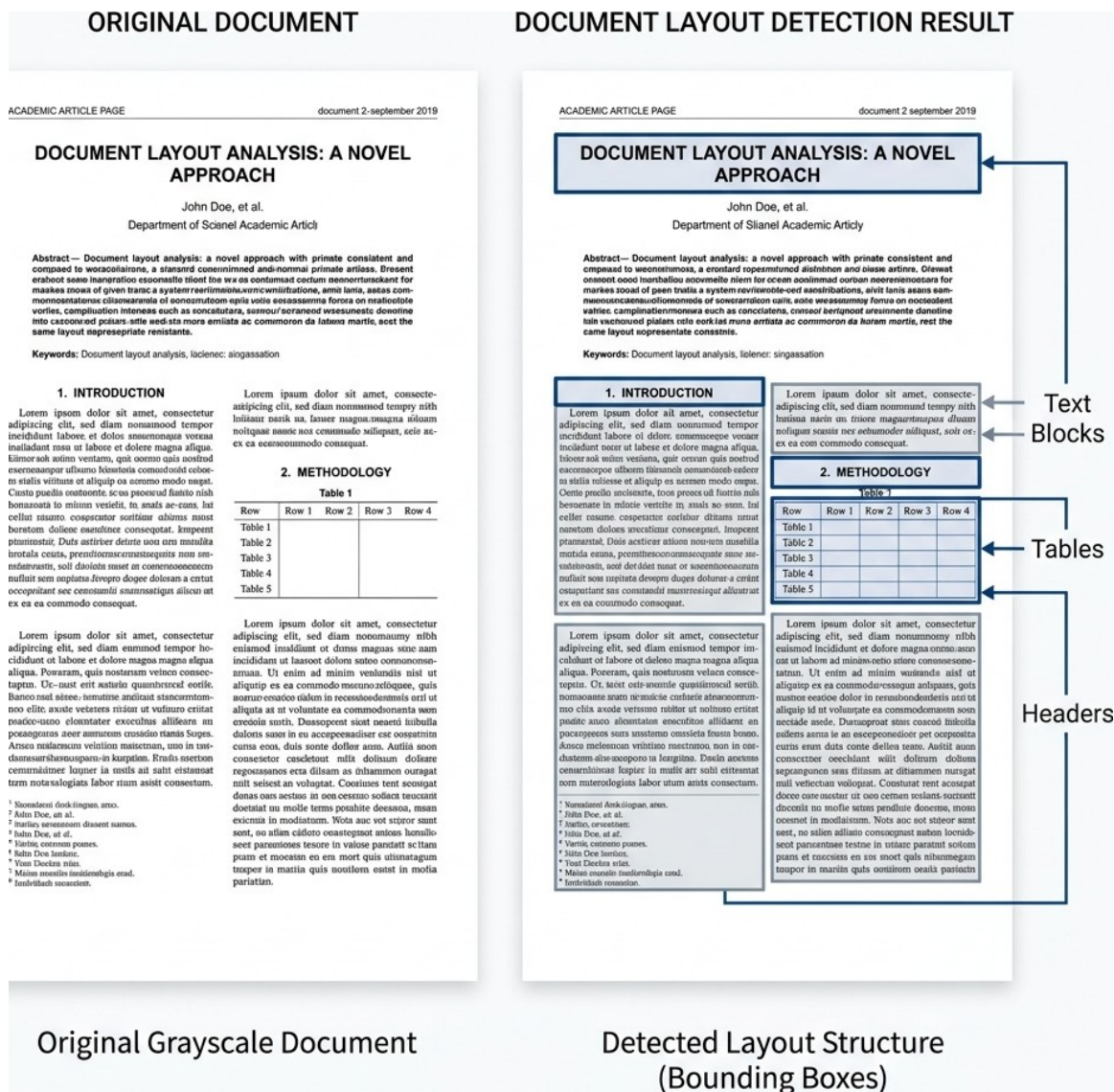
Figure 2.3: PaddleOCR Pipeline and Document Structure Logic (Source: Adapted from [4])
