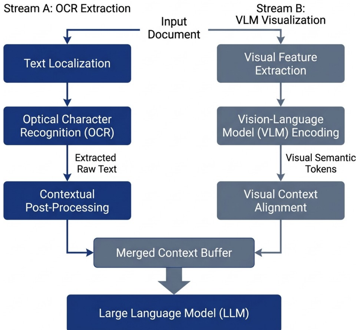
Figure 4.3: Dual-Stream Synchronization Principle (Source: Own elaboration)
