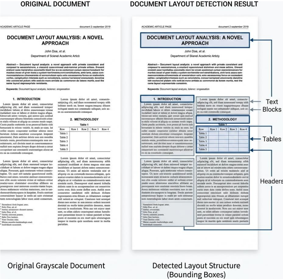
Figure 2.3: Layout Detection and Document Structure Logic
