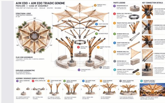
AIMV-004 EDO triadic pavilion - kit of assembly
