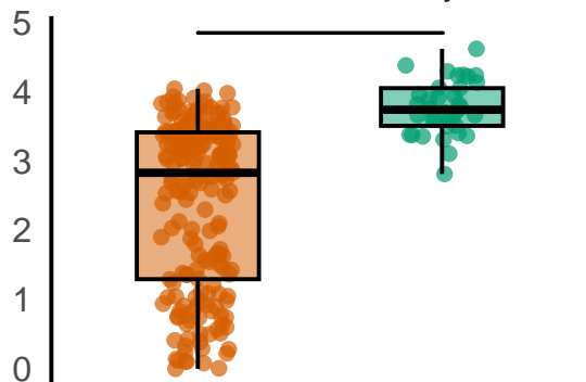
Shannon Diversity
