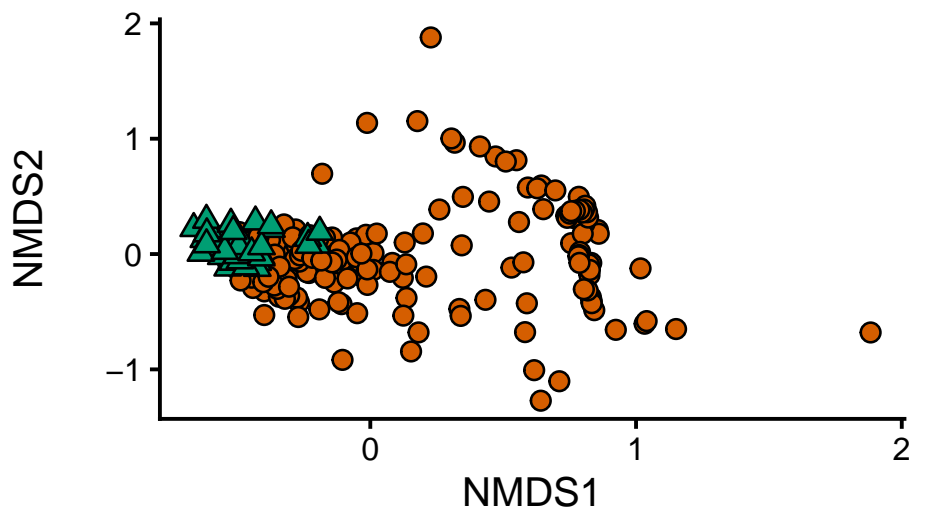
NMDS (Bray-Curtis) – stress=0.19
