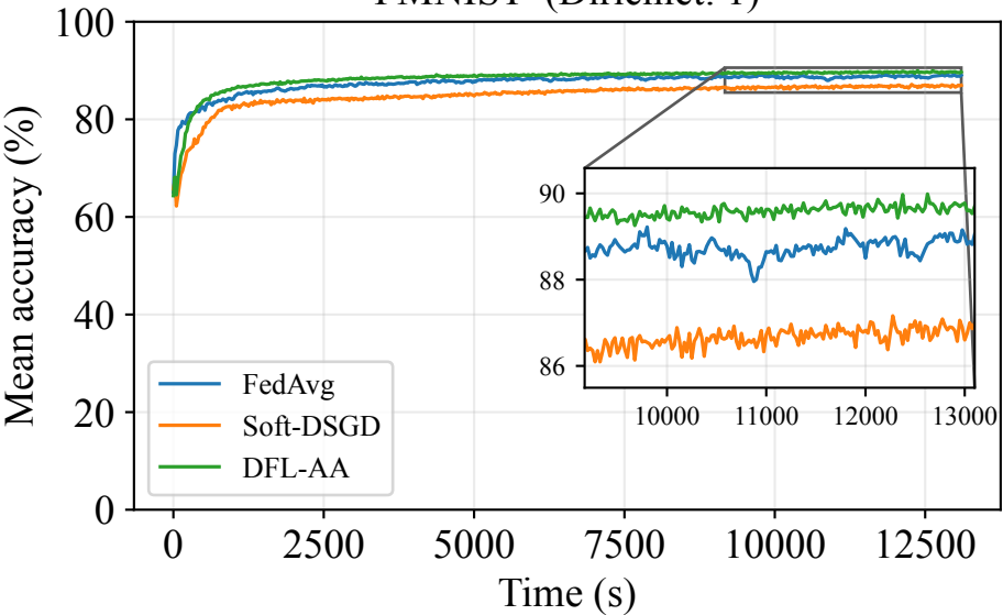
FMNIST (Dirichlet: 1)
