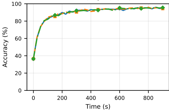
MNIST ( \alpha=0.1 )
