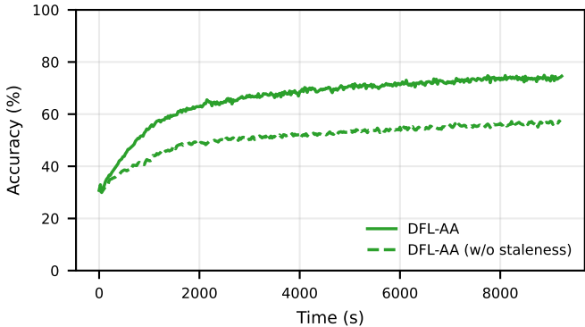
FMNIST ( \alpha=0.1 )
