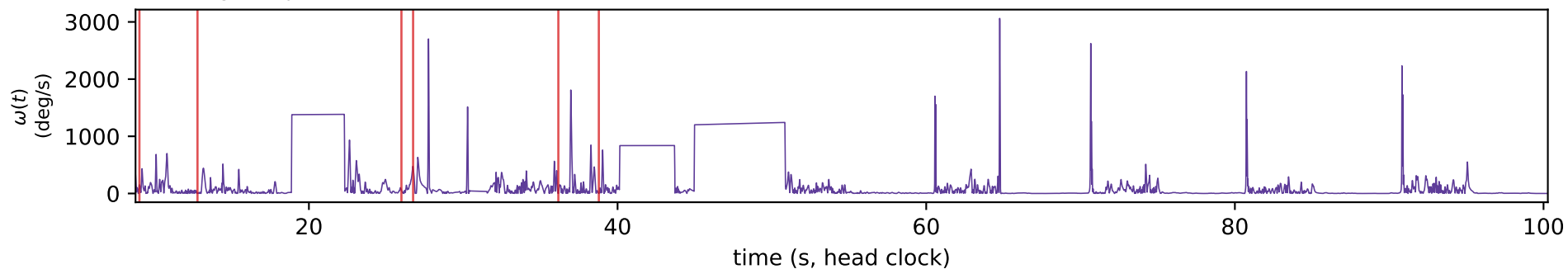
Head angular speed \omega(t) ; red = bout onsets
