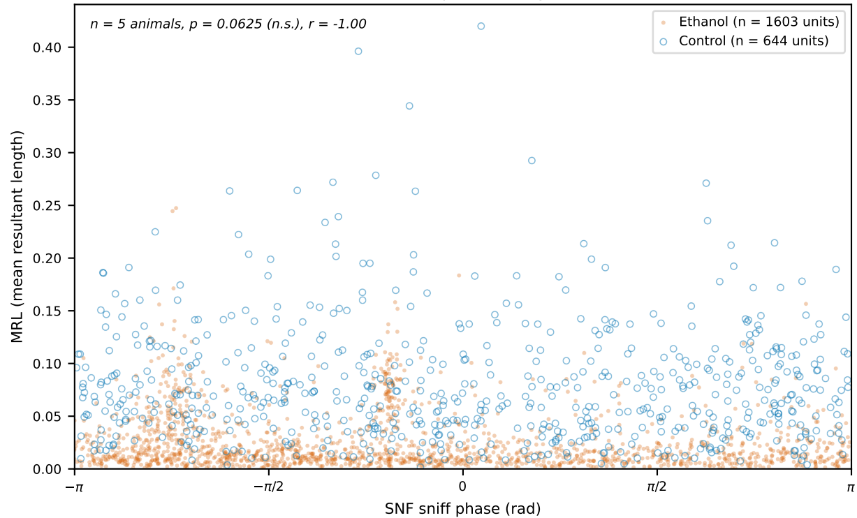
Per-unit phase-locking
