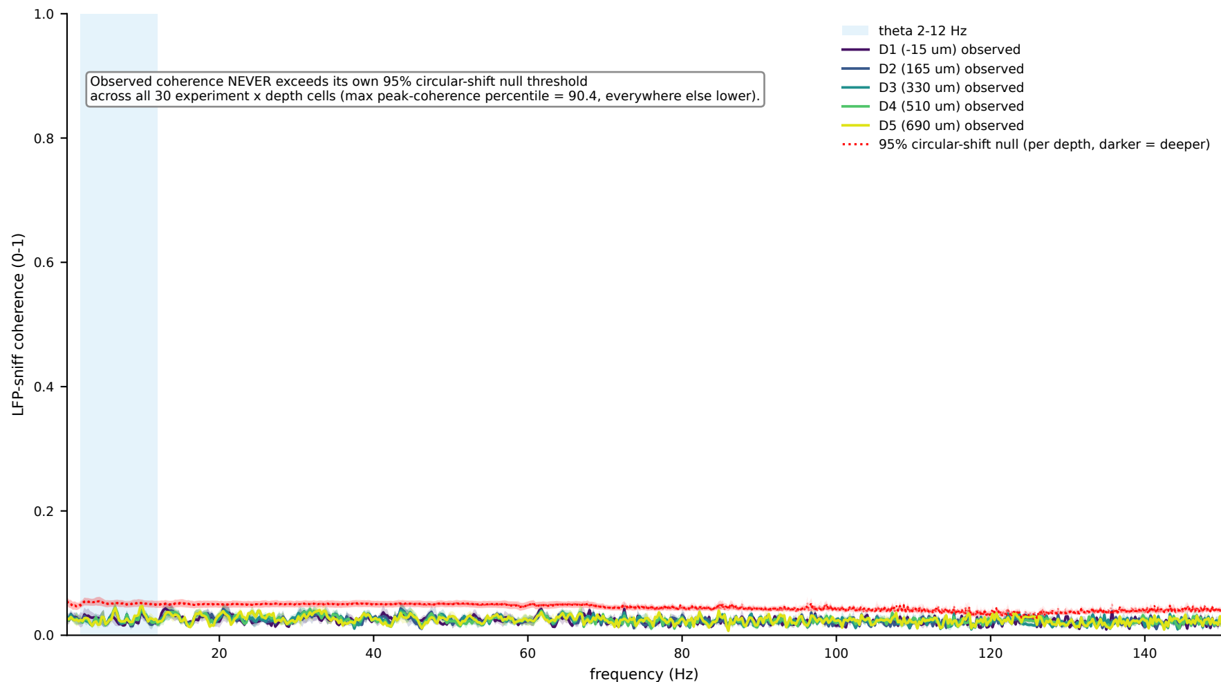
Figure 1C-bottom / 1E analogue (KEY): LFP-sniff coherence spectrum per depth with null threshold
