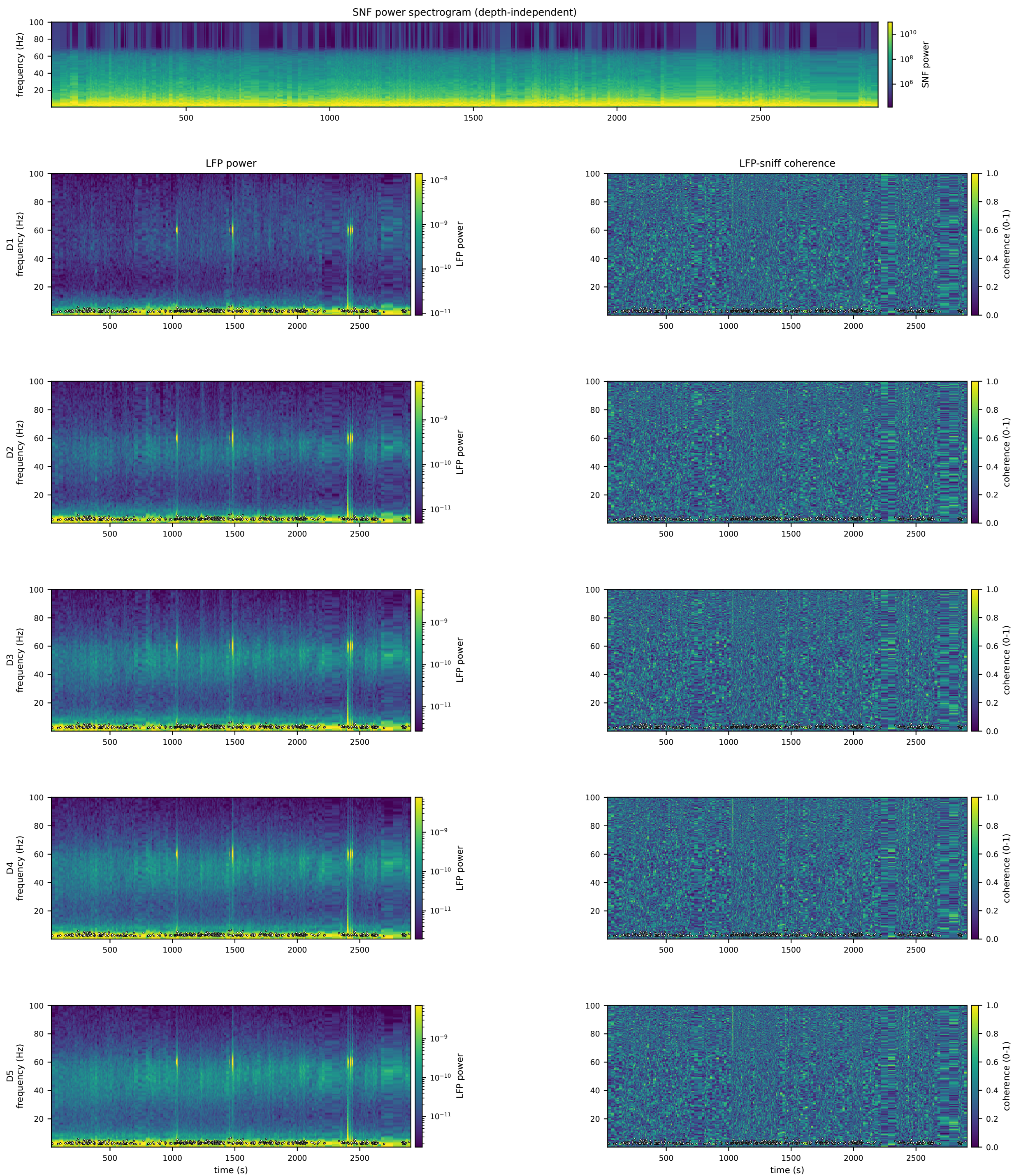
Figure 1C analogue: multitaper spectrograms per depth with sniff-rate overlay. Representative experiment: session 06-24-2022 (same session/display convention as FIG-PAPER1-TRACES); full recording duration shown (not restricted to the 10-s FIG-PAPER1-TRACES segment). Depth channels: D1=ch0 (-15 \mu m), D2=ch24 (165 \mu m), D3=ch46 (330 \mu m), D4=ch118 (510 \mu m), D5=ch142 (690 \mu m). multitaper: 4-s windows, 50% overlap, 7 Slepian tapers (NW=4), freqs \geq 0.25 Hz. Colorbars: LFP power, SNF power, coherence (0-1). White/black-edged scatter overlay = instantaneous sniff rate (Hz). Frequency axis cropped to 0-100 Hz for display; underlying data extend to 500 Hz.
