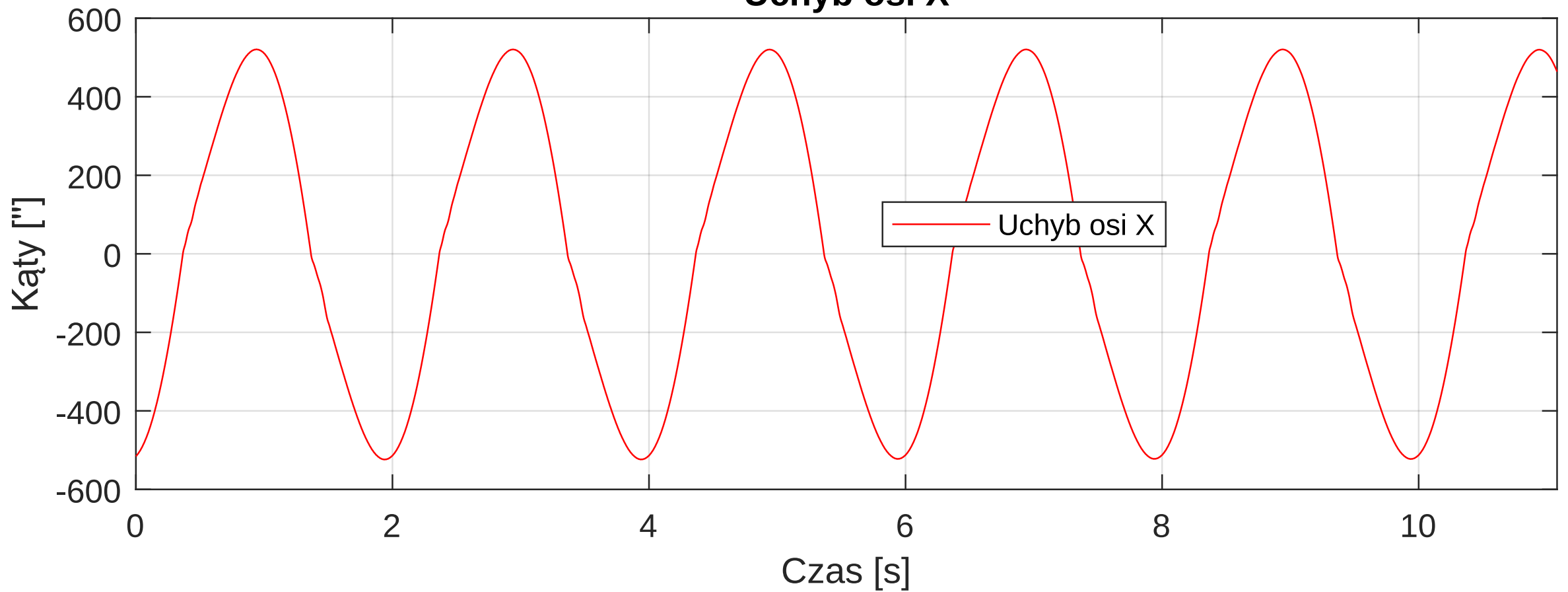
Uchyb osi X
