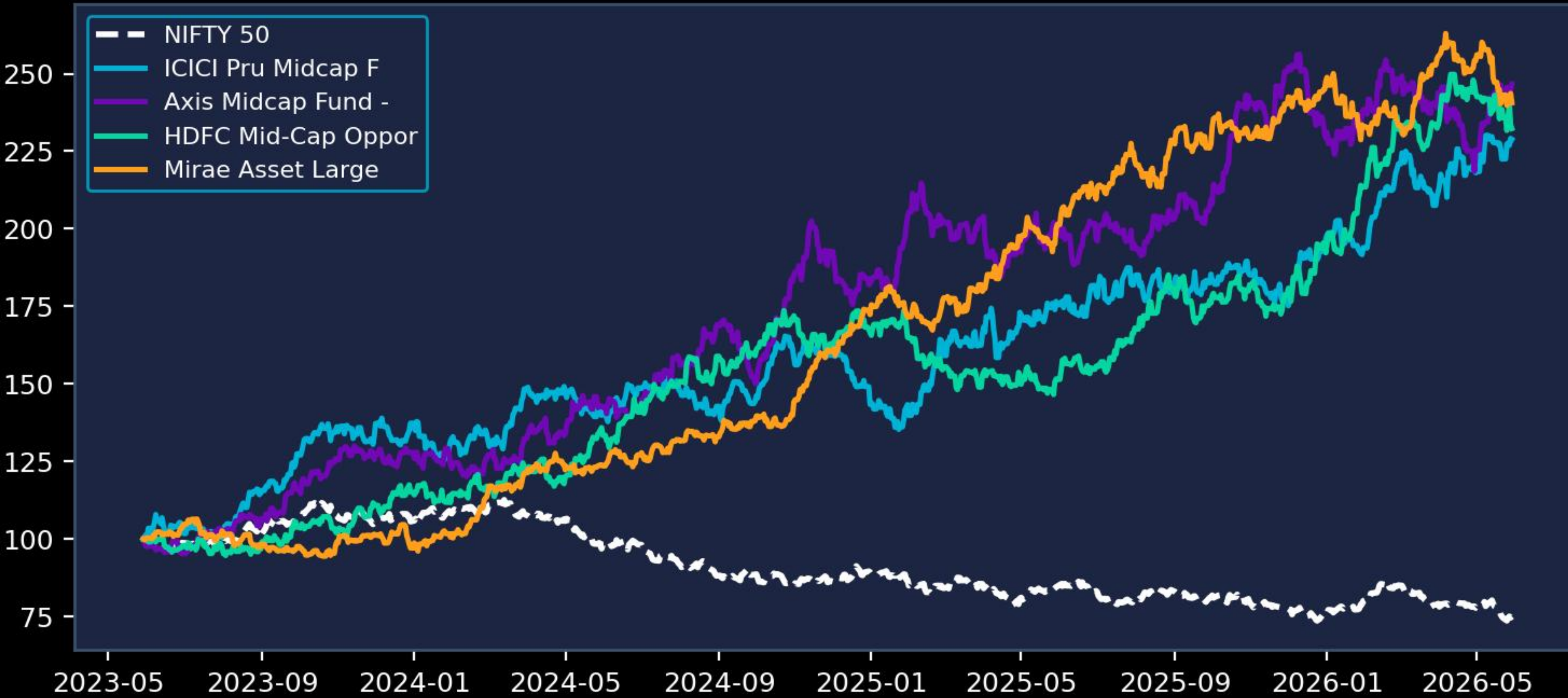
Top 5 Schemes NAV Progression vs NIFTY 50 Benchmark
