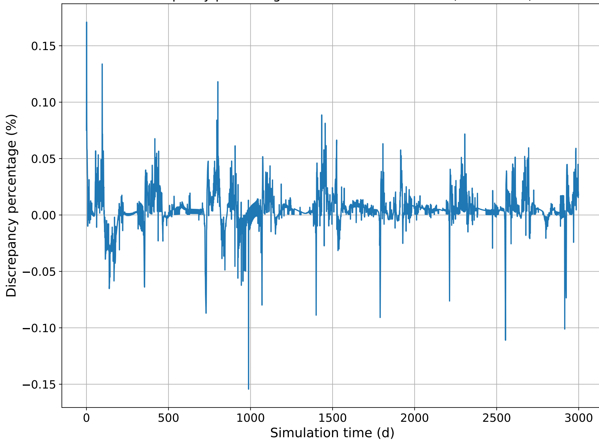
Discrepancy percentage of the MODFLOW model (flow model)
