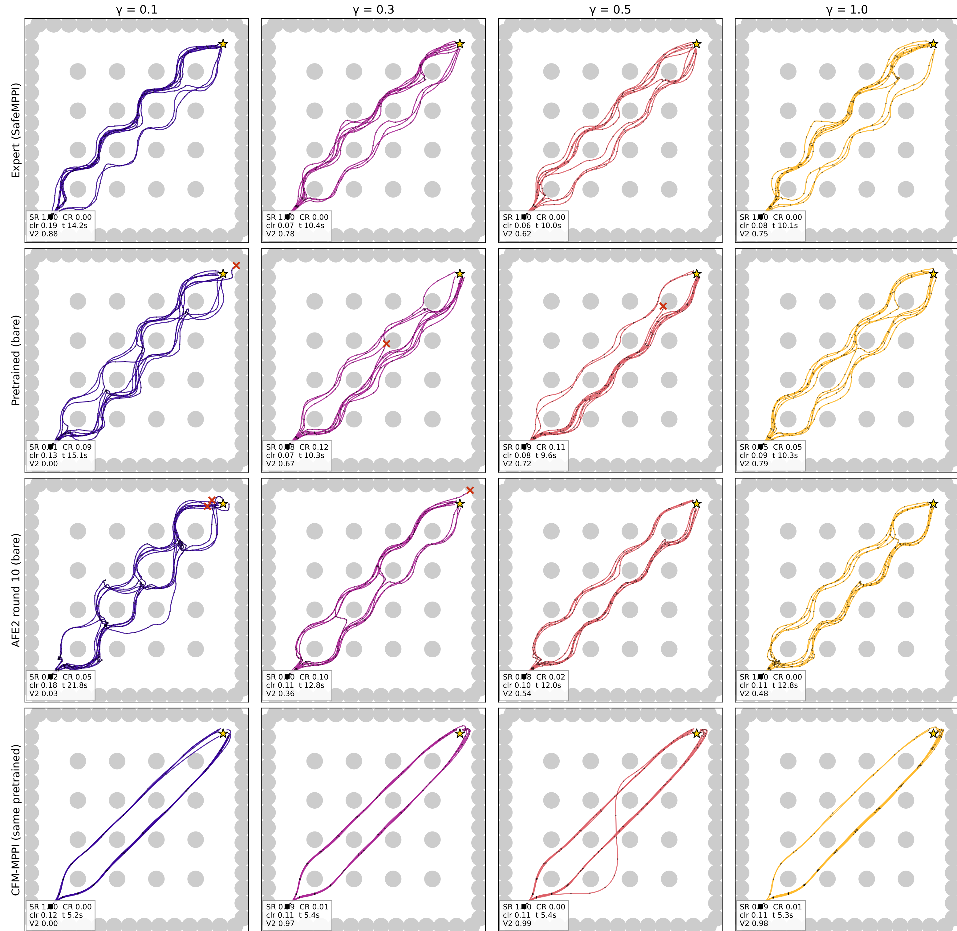
TRUE evaluation — M=100 random rollouts per cell; each panel shows 10 ratio-matched random trajectories (no curation)
