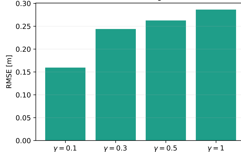
Position-tracking RMSE
